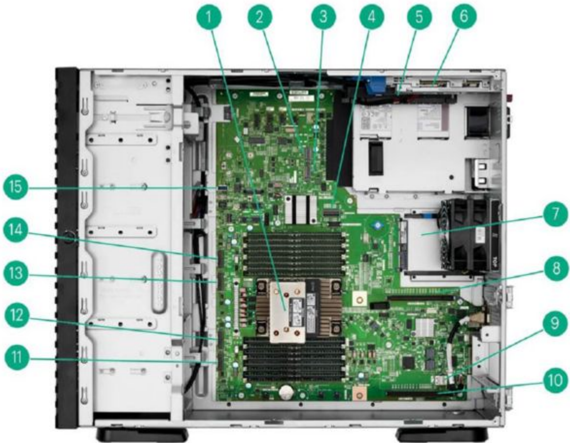
Internal View - with full memory DIMM populated, and optional NS204i-u shown
